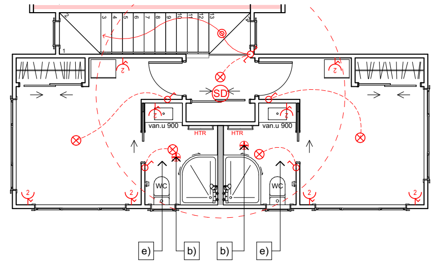
Upper Electrical Plan
