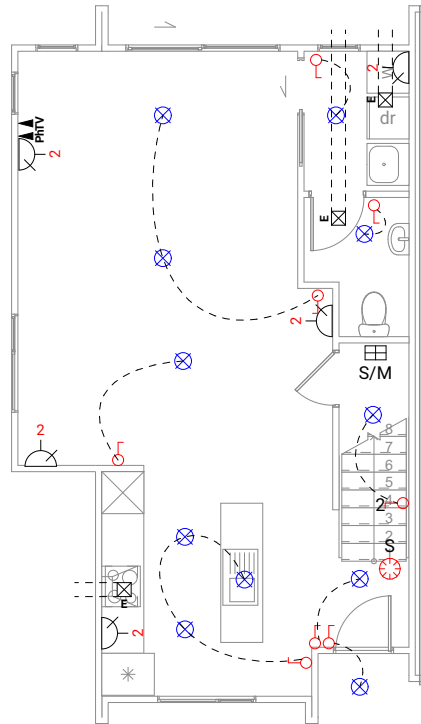
Lower Electrical Plan
