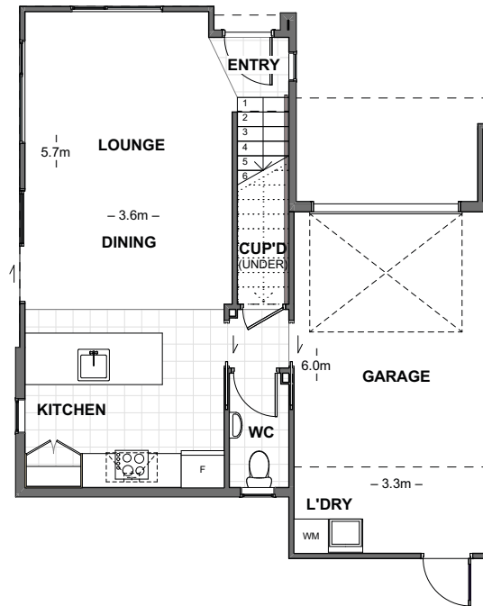
LOWER LEVEL FLOOR PLAN 61.75m 2
