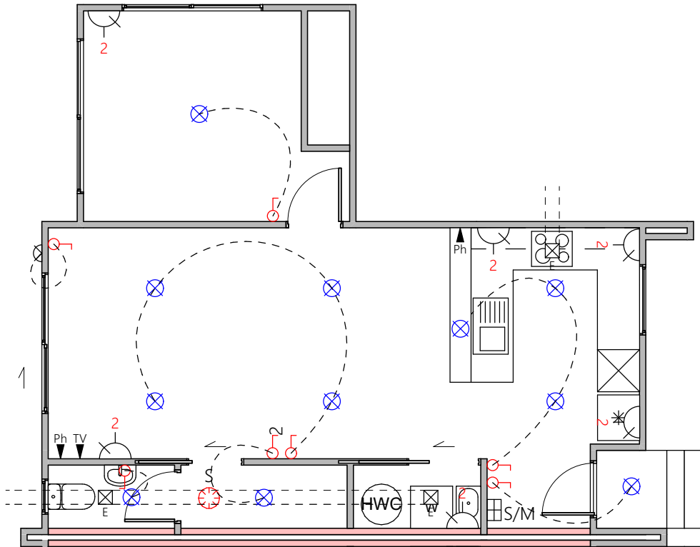
Lower Electrical Plan
