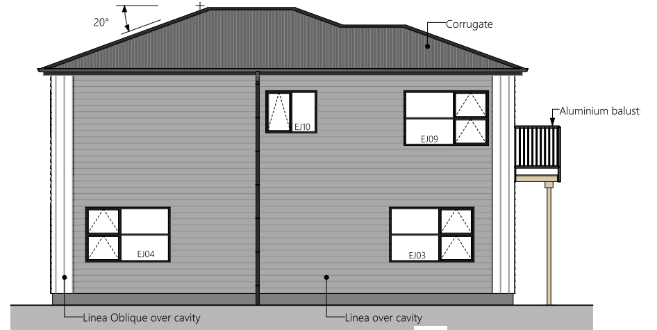
2 North Elevation
