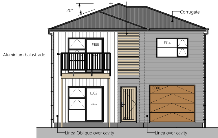
1 West Elevation
