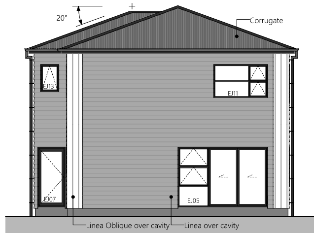
3 East Elevation
