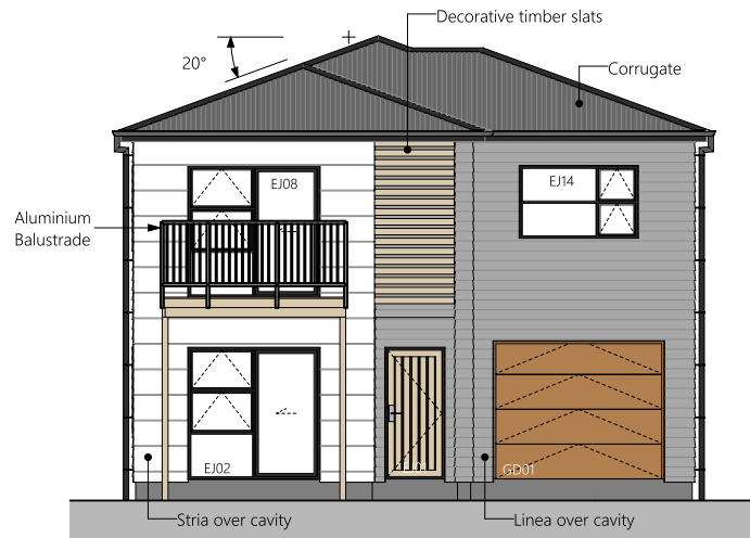
1 West Elevation
