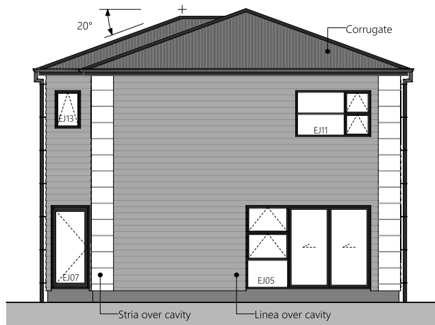
3 East Elevation
