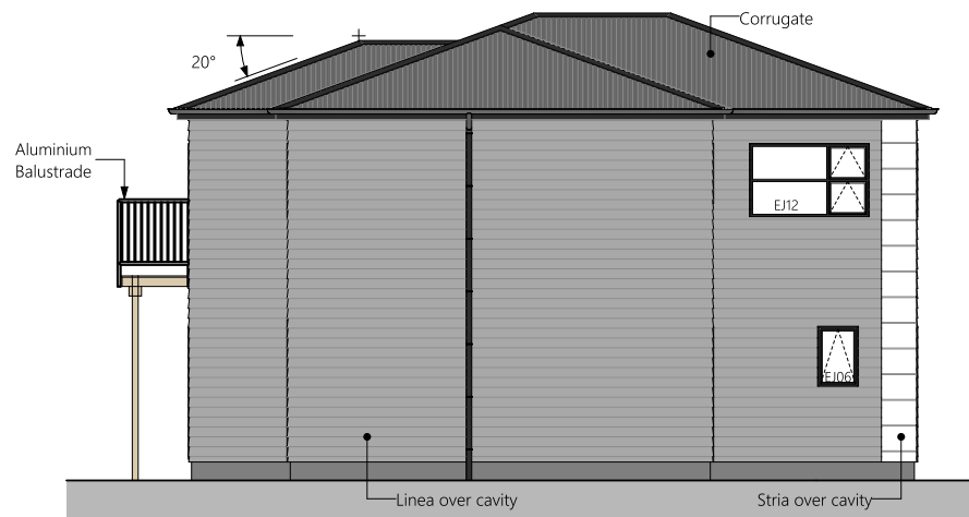
4 South Elevation
