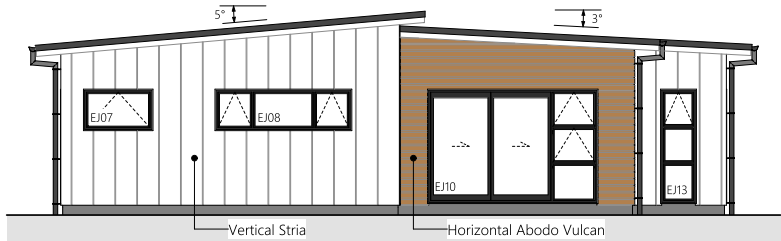
3 North Elevation
