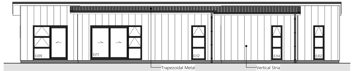
4 West Elevation
