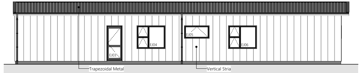
2 East Elevation
