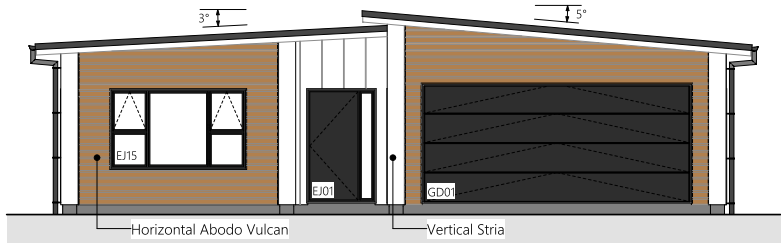
1 South Elevation
